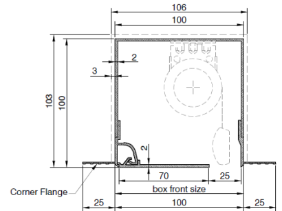
Head Box W100x100 S
