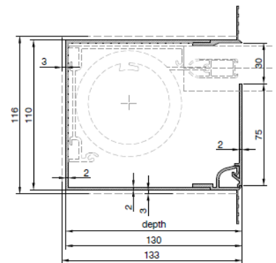
Head Box R110x130 S
