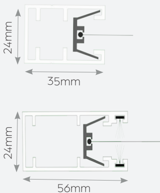
FABRIC RETENTION SIDE CHANNELS
