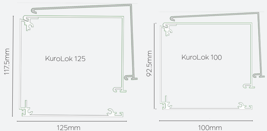
KUROLOK HEADBOX DIMENSIONS
